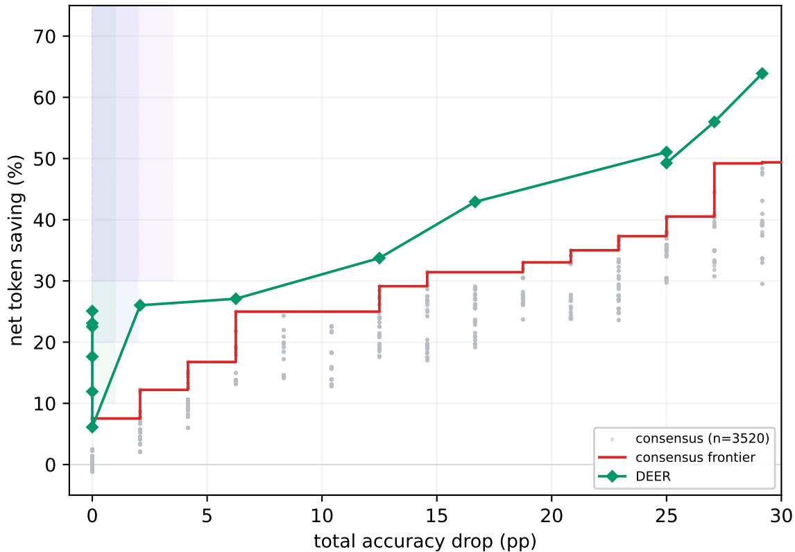
amc23 (dev)
