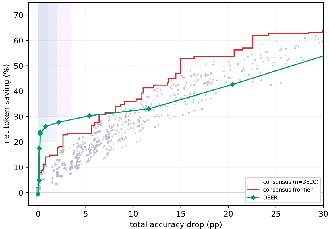
DeepSeek-R1-Distill-Qwen-7B (dev)
