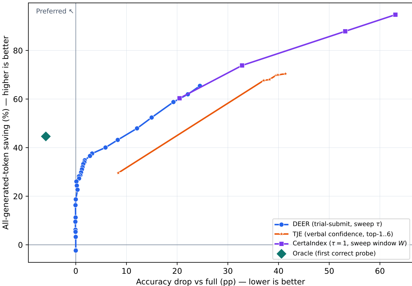
Vanilla early-exit signal frontiers Macro (mean over the three benchmarks)
