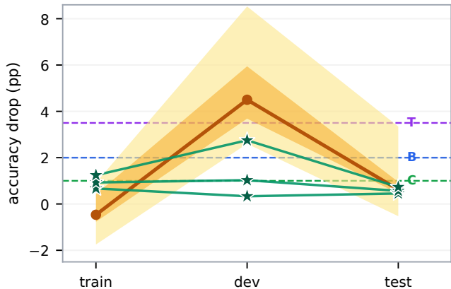
Accuracy drop
