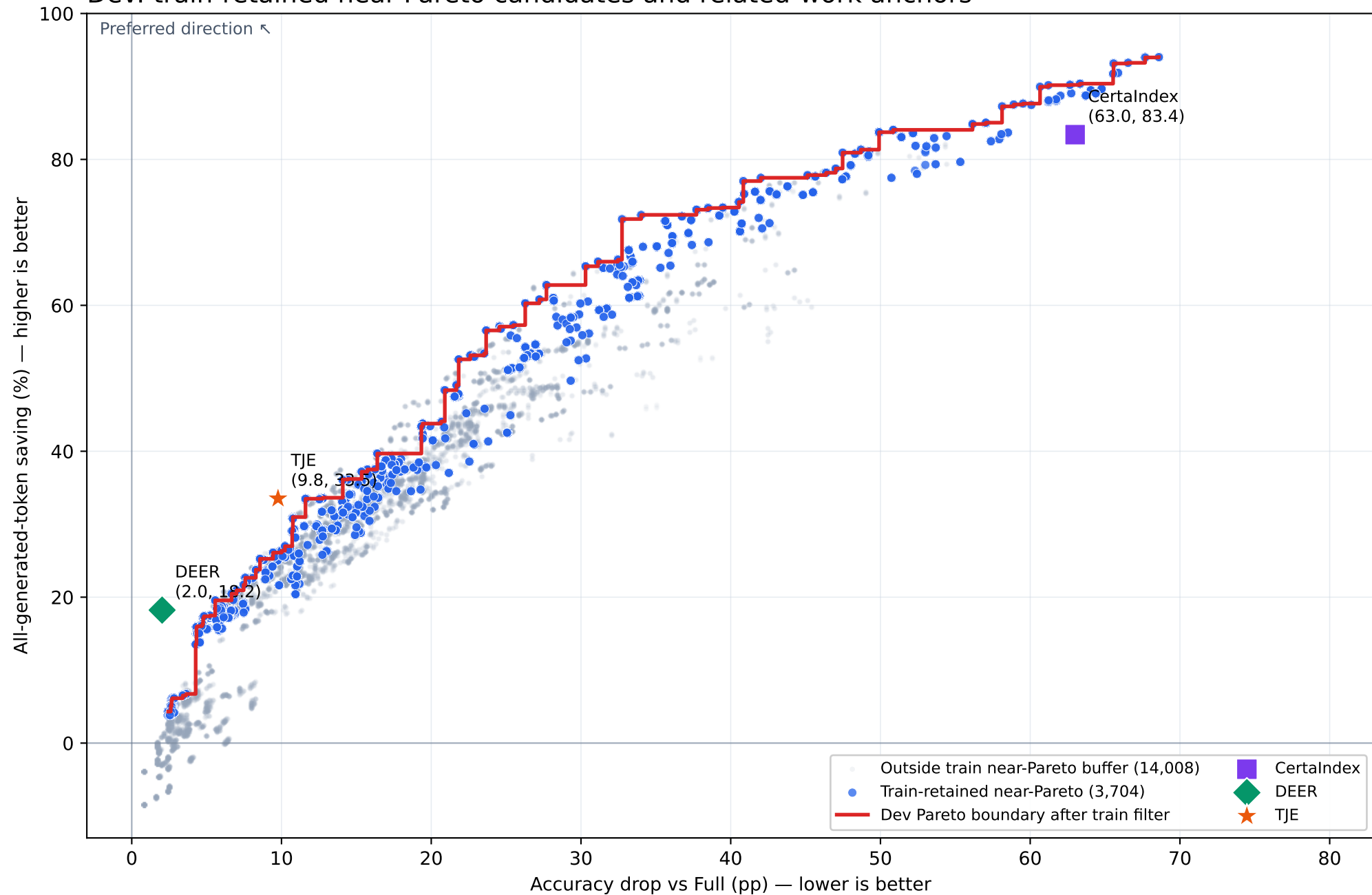
Dev: train-retained near-Pareto candidates and related-work anchors
