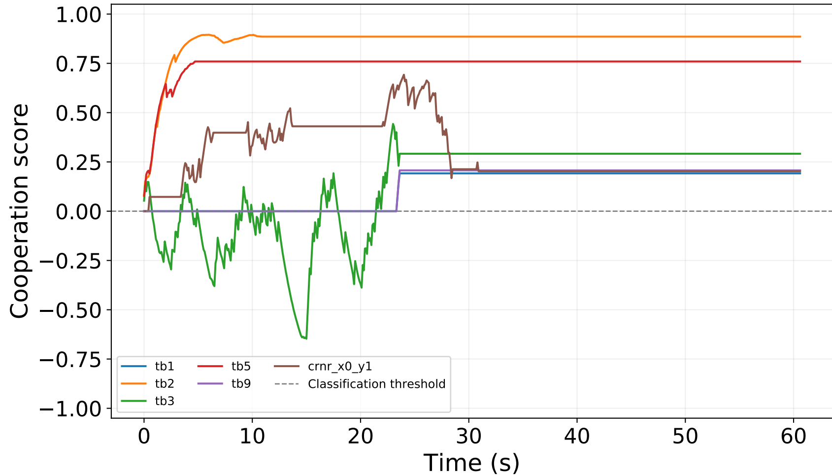
tb6 — per-neighbor cooperation
