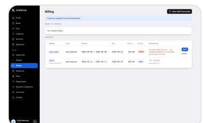
Billing: an invoice Procountor refused (Send retries it) and one it has collected.
