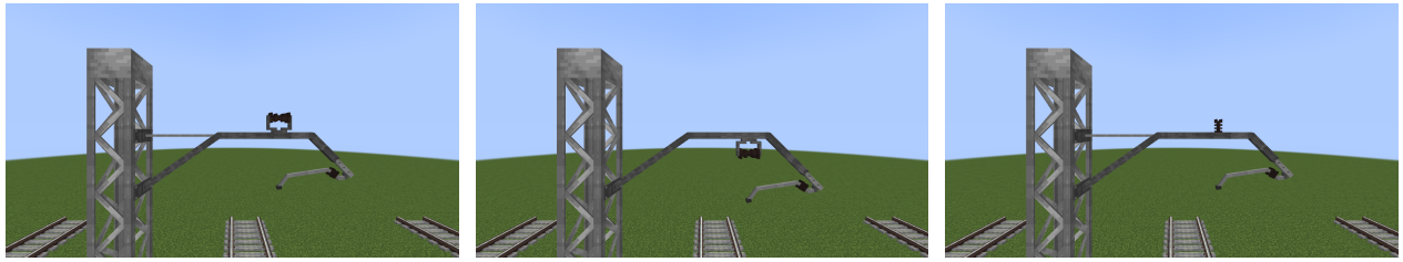
(a) Horizontal support: the messenger rests on top of a horizontal insulator. (b) Horizontal hanging support: the insulator hangs below the tube (shown without support wire). (c) Vertical support: a vertical insulator on top of the tube.
