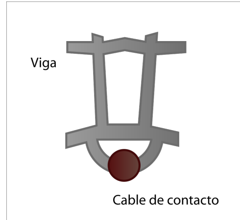
(b) Cross-section of a rigid catenary profile ( viga ) with the contact wire ( cable de contacto ) clamped below.
