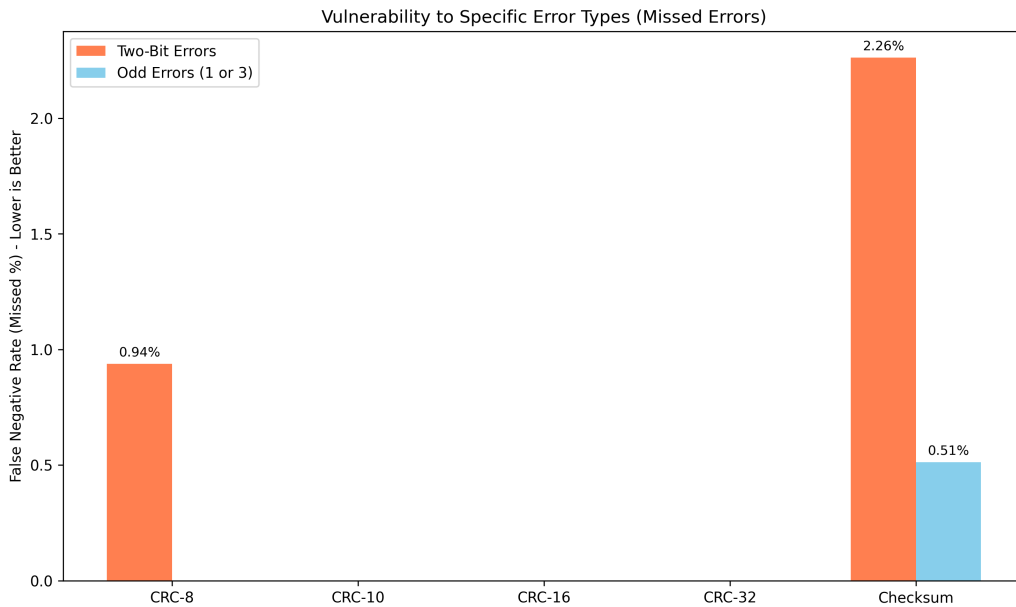
Figure 7: False negative (missed error) rate for the vulnerable methods.
