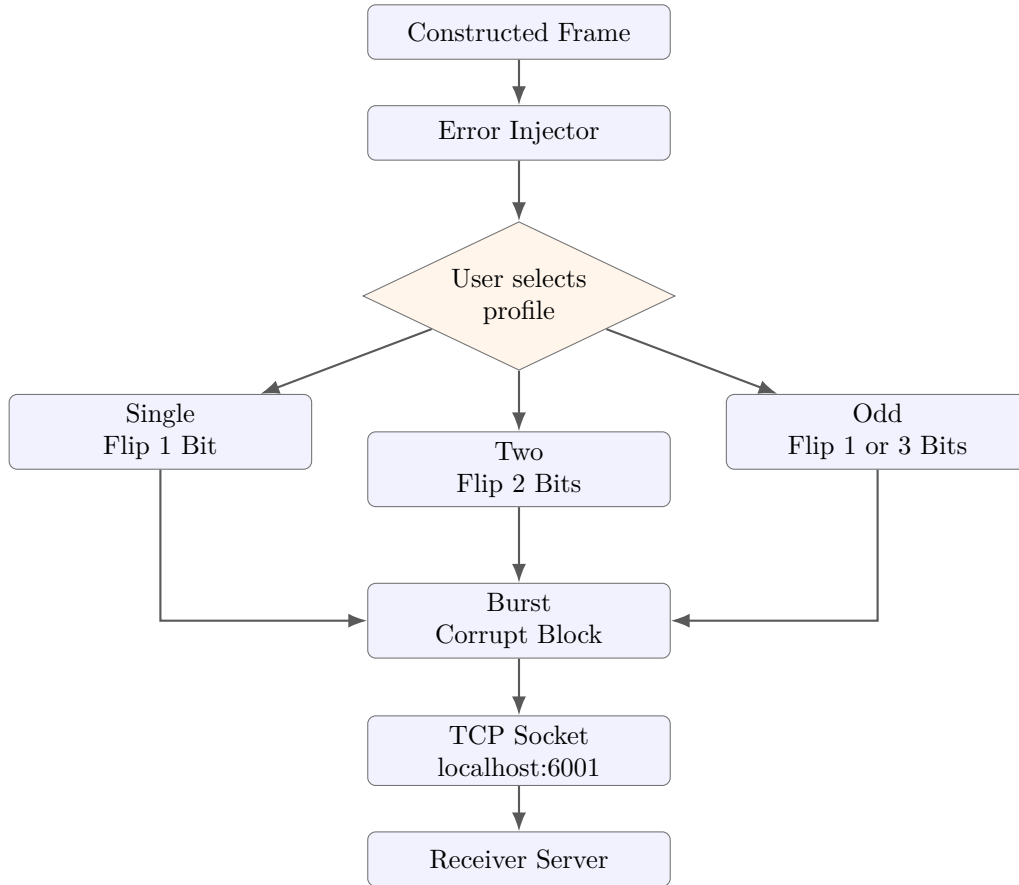
Figure 2: Error profile selection and transmission over the TCP socket.
