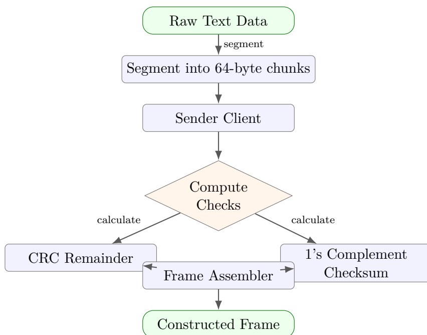
Figure 1: Frame construction at the sender: from raw data to a checked, assembled frame.
