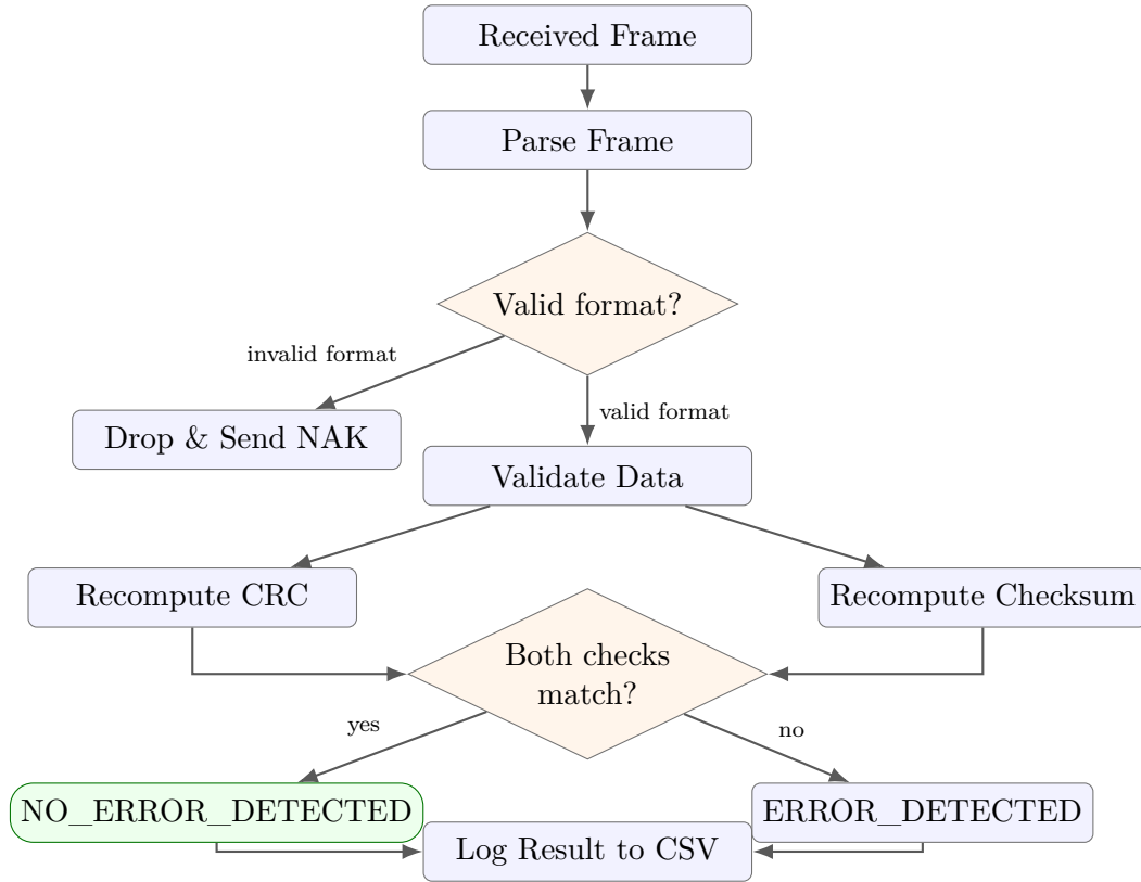
Figure 3: Parsing, dual validation, and outcome logging at the receiver.
