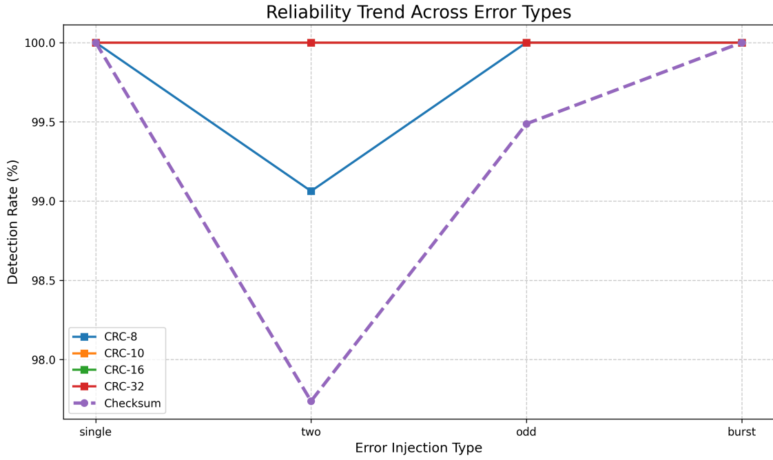
Figure 6: Reliability trend of each detection method across error injection types.
