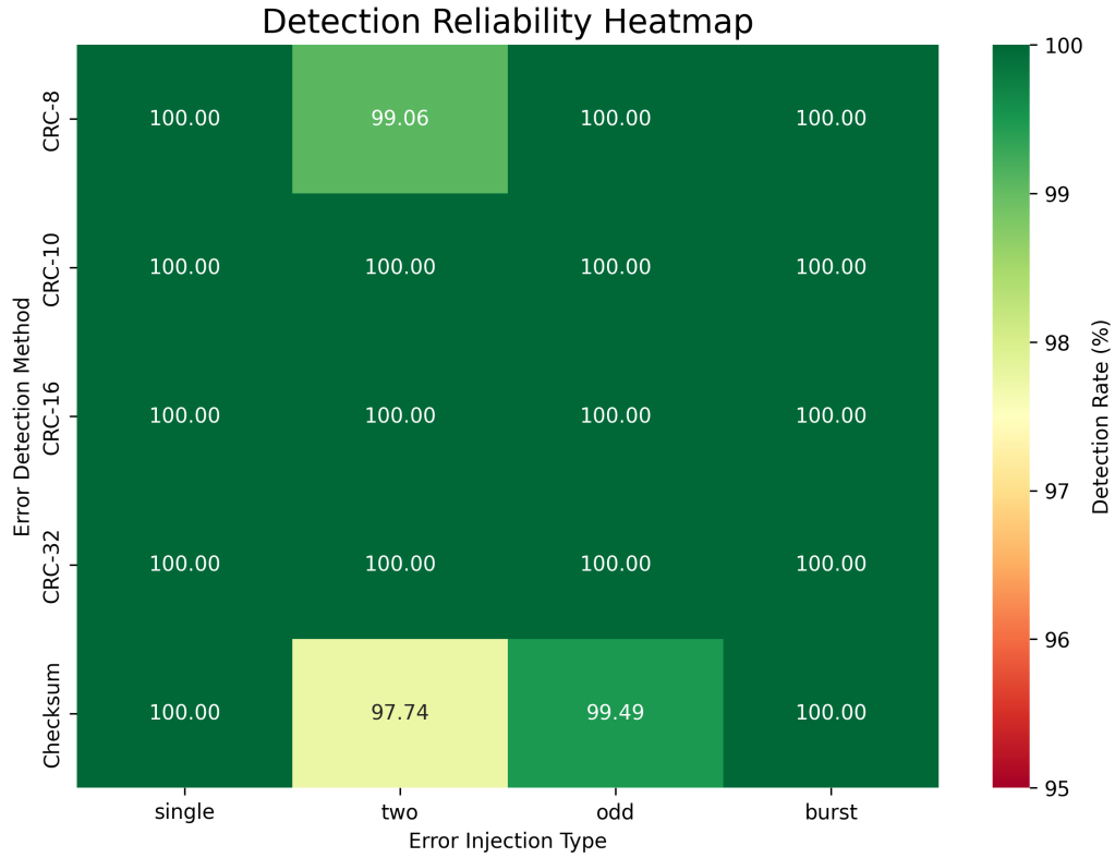
Figure 4: Detection reliability heatmap across all polynomials and error types.
