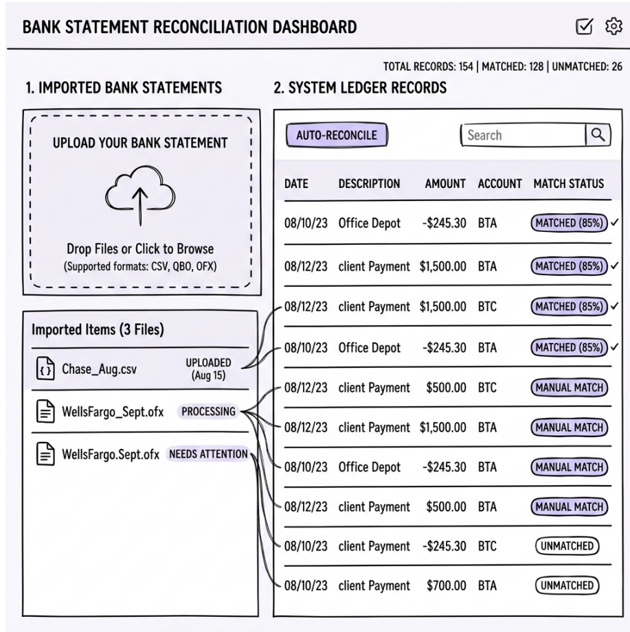
Figure 7: Proposed Bank Reconciliation Tool UI Wireframe
