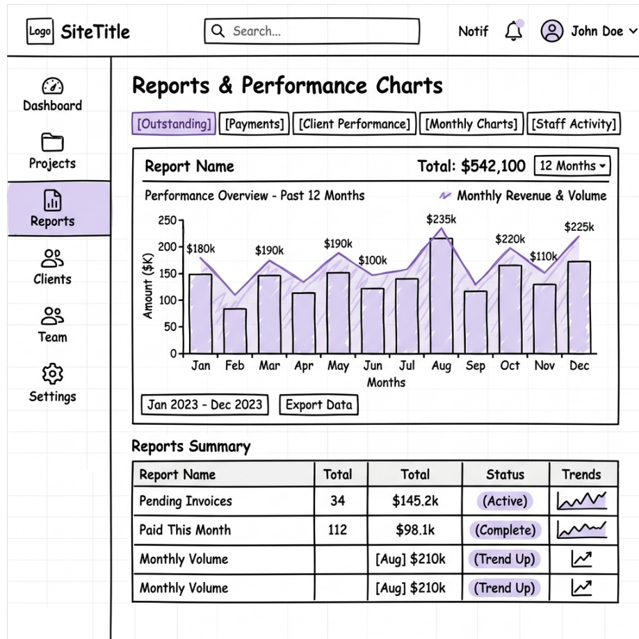
Figure 5: Reports and Chart Panel (/reports) Screen Layout
