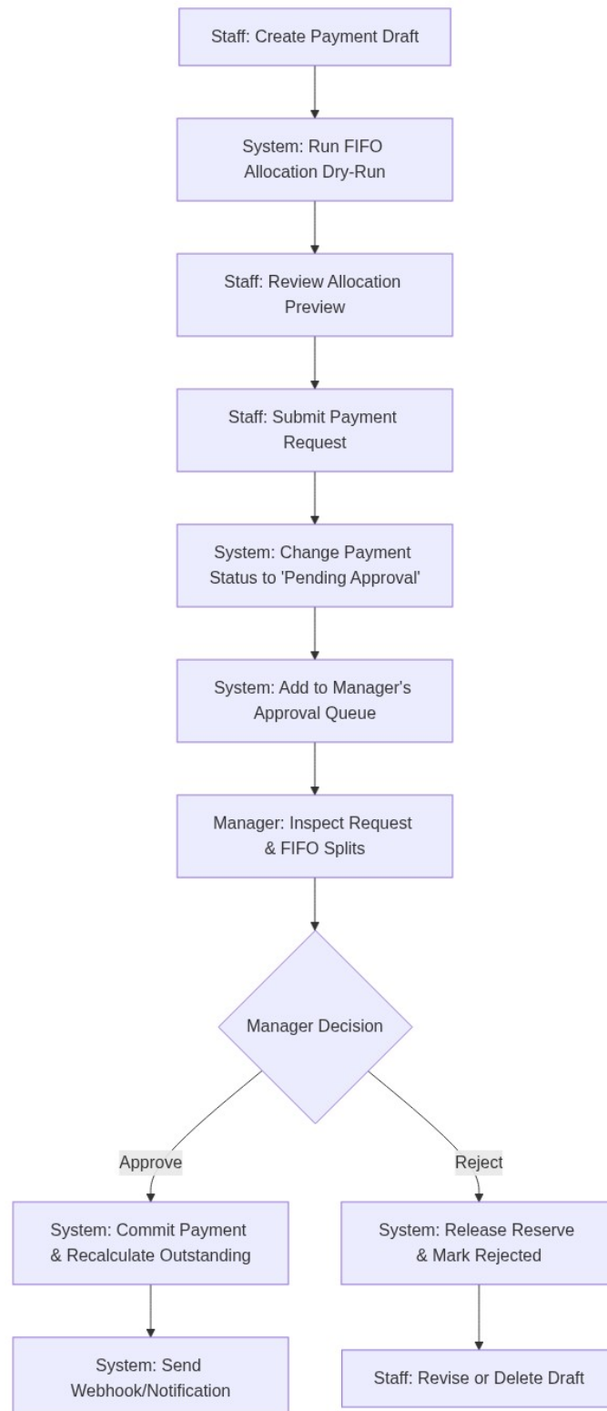
Figure 9: Proposed Maker-Checker Payment Approval Lifecycle
