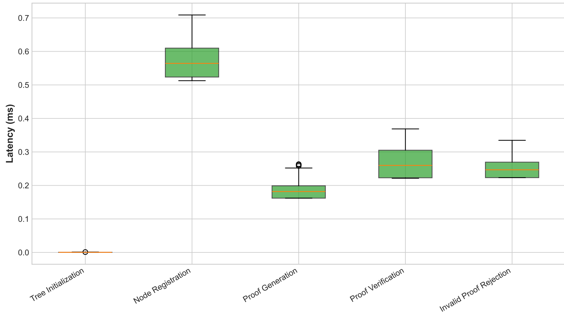
SMT Microbenchmarks — Latency Distribution (Box Plot)
