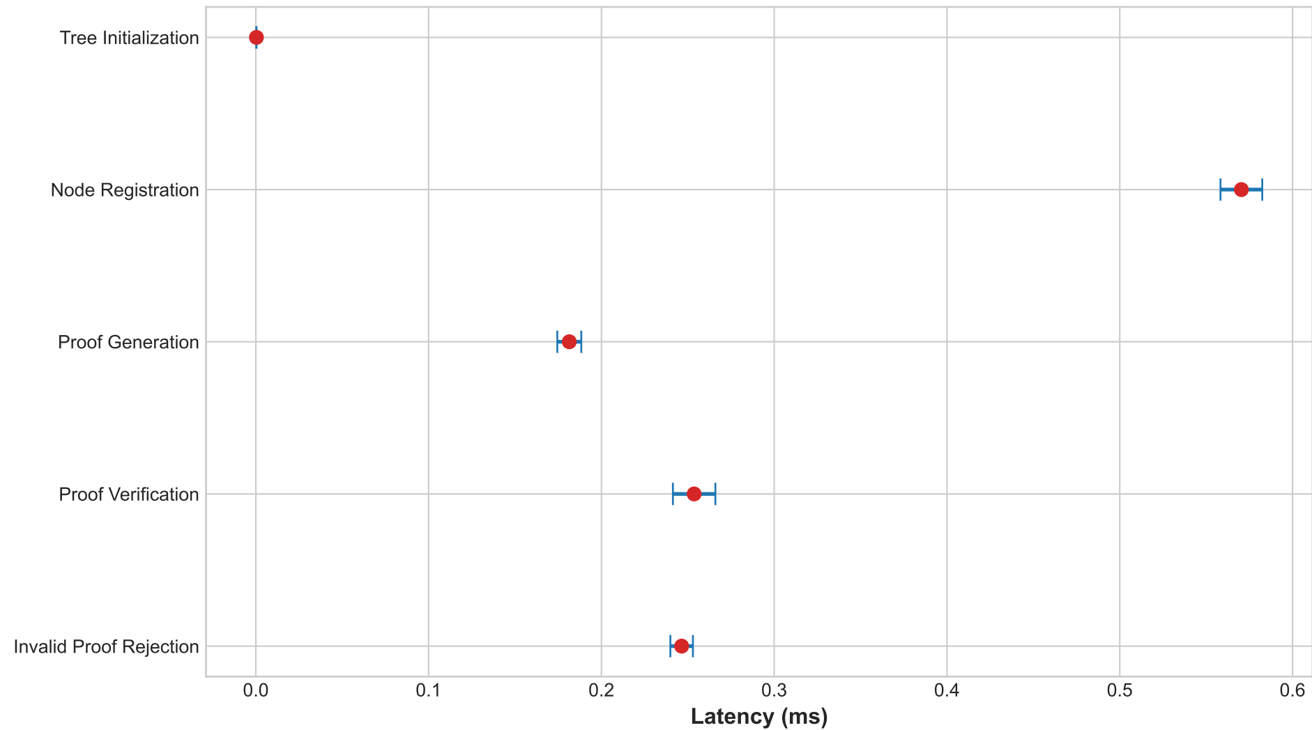
SMT Microbenchmarks — Mean & 95% Confidence Intervals
