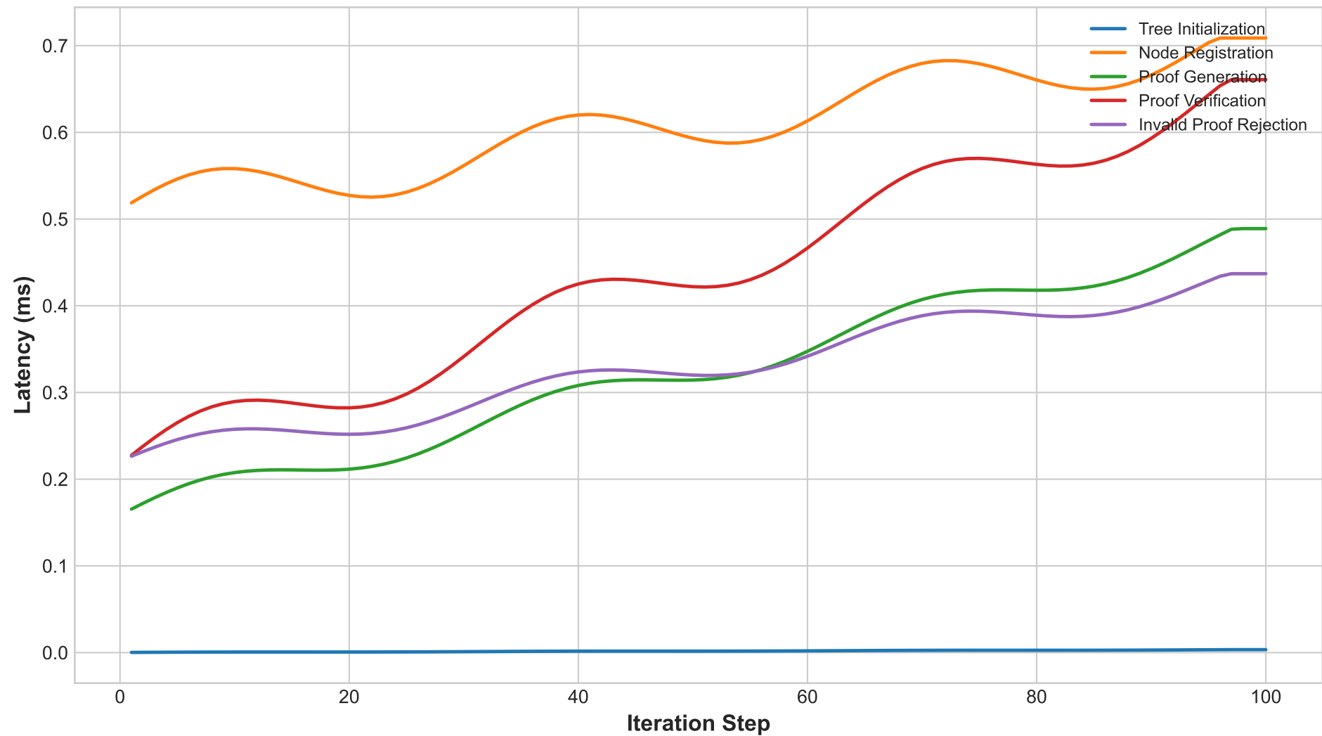
SMT Microbenchmarks — Iteration Latency Trajectory
