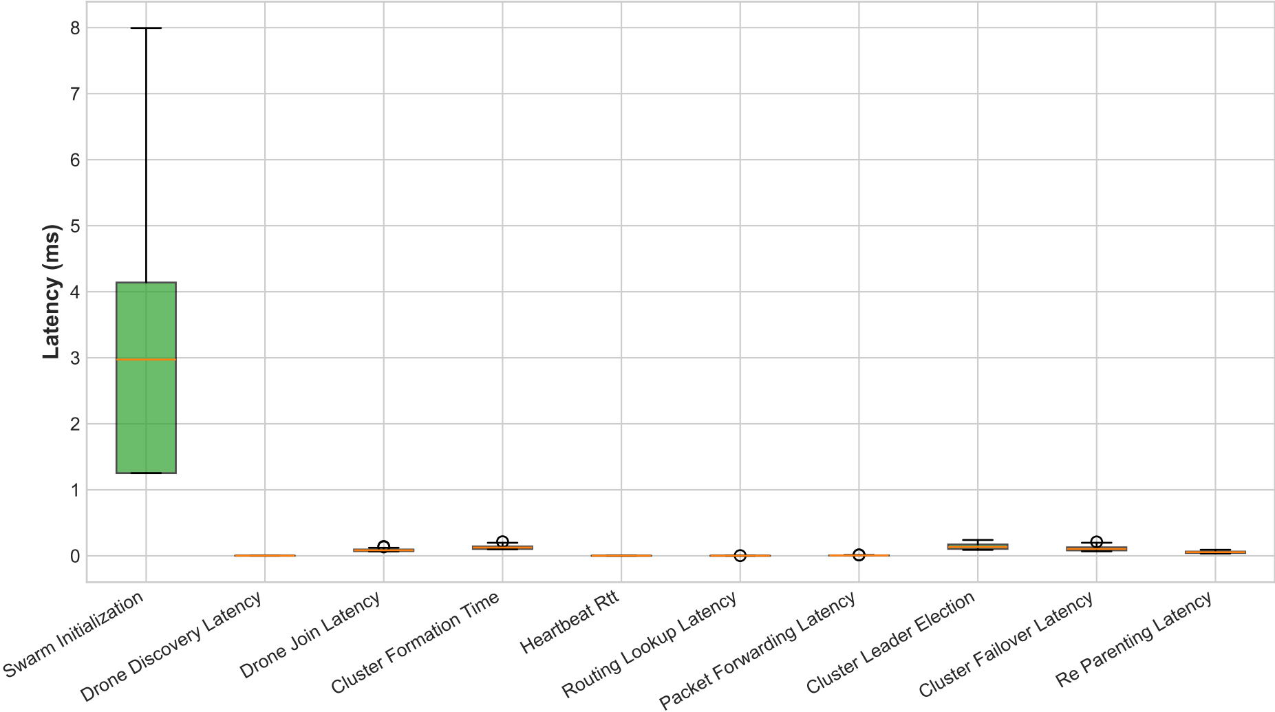
Hierarchical Swarm Microbenchmarks — Latency Distribution (Box Plot)
