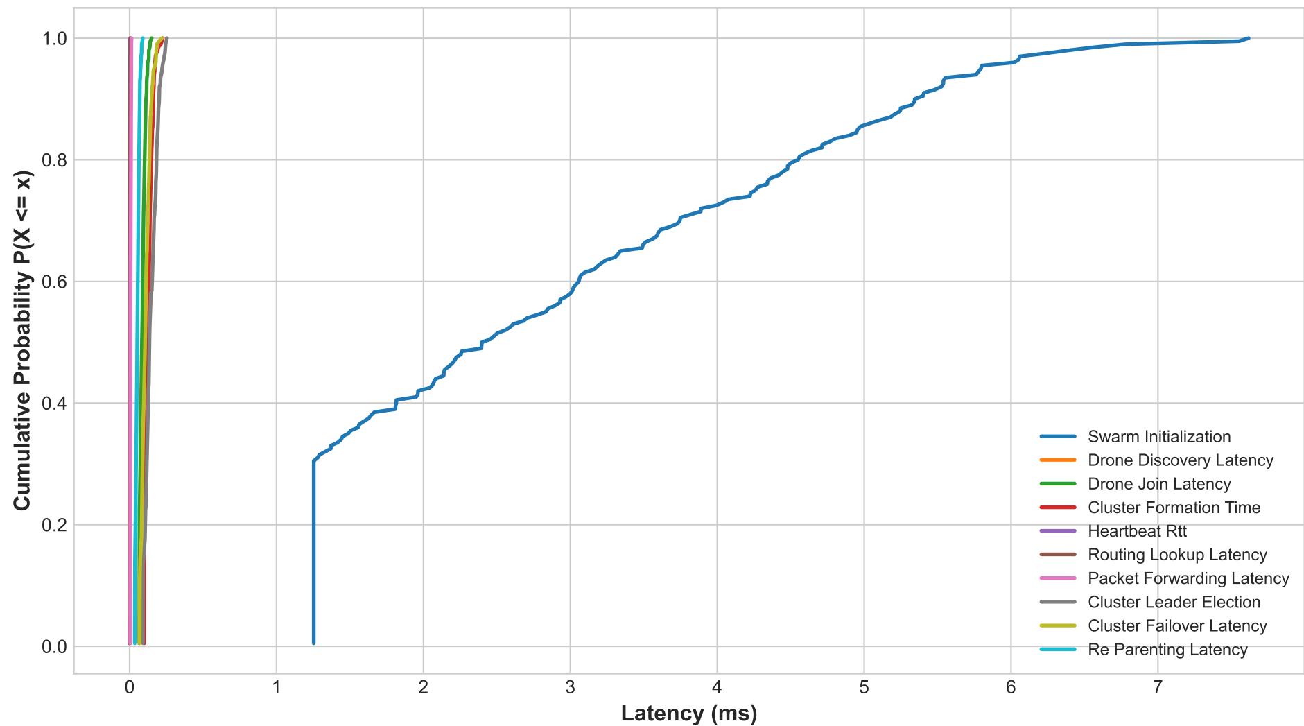
Hierarchical Swarm Microbenchmarks — Cumulative Distribution Function (CDF)
