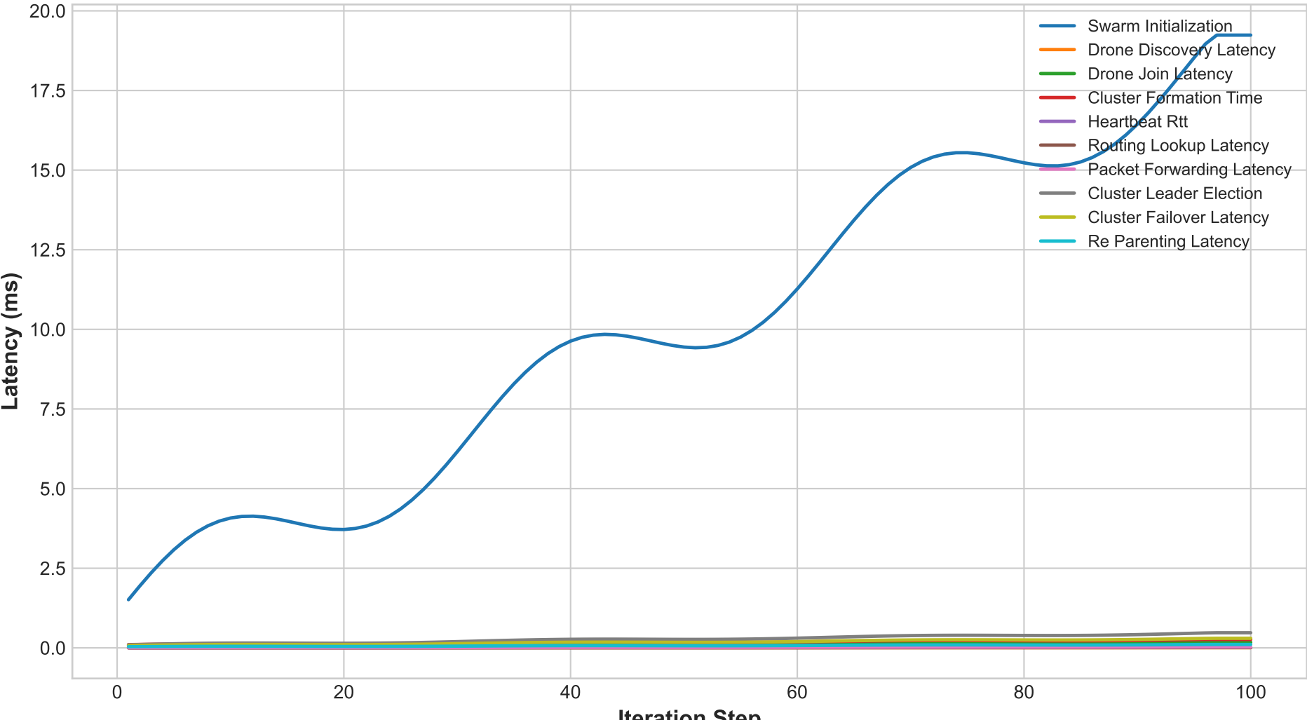
Hierarchical Swarm Microbenchmarks — Iteration Latency Trajectory
