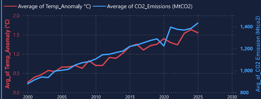
Average of Temp_Anomaly °C and Average of CO2_Emissions (MtCO2) by year
