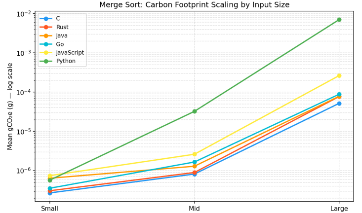
Figure 7: Mean gCO 2 e for merge sort by language and input size, with large/small scaling ratio.
