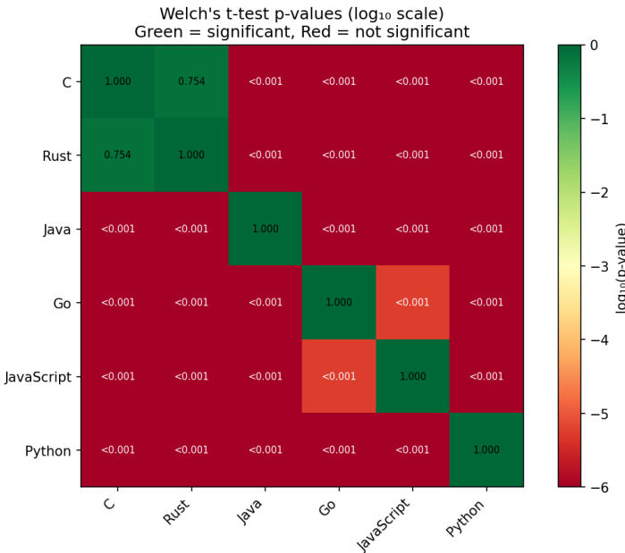
Figure 3: P-value heatmap for pairwise language comparisons (large input size).
