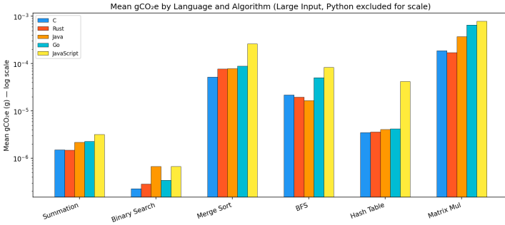
Figure 5: Mean gCO 2 e per measurement by language and algorithm (log scale; Python excluded).
