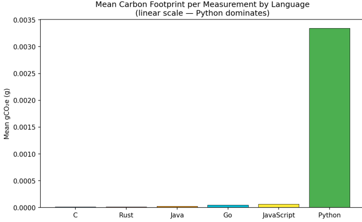
Figure 2: Mean gCO 2 e per measurement by language (linear scale).
