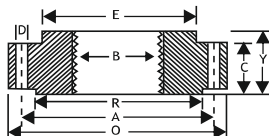
THREADED FLANGE
