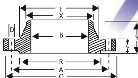
WELDING NECK FLANGE
