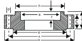
SOCKET WELD FLANGE
