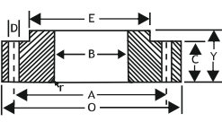
LAP JOINT FLANGE
