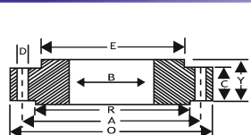
SLIP-ON FLANGE
