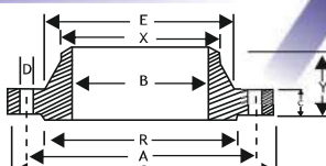
WELDING NECK FLANGE
