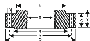
THREADED FLANGE
