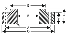
LAP JOINT FLANGE
