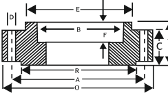
SOCKET WELD FLANGE
