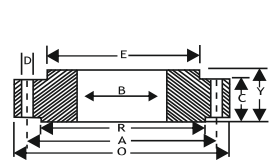
SLIP-ON FLANGE
