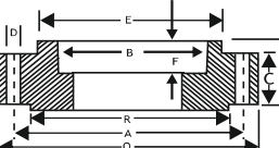
SOCKET WELD FLANGE
