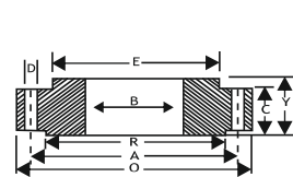
SLIP-ON FLANGE
