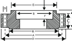
SOCKET WELD FLANGE
