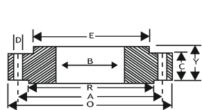
SLIP-ON FLANGE
