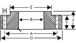
LAP JOINT FLANGE
