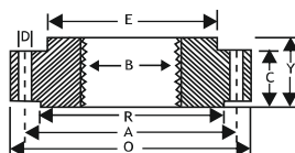
THREADED FLANGE
