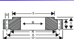
SLIP-ON FLANGE
