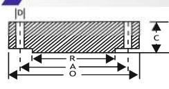
BLIND FLANGE
