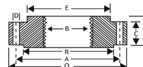
THREADED FLANGE
