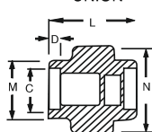
SOCKET WELD FITTING TO ANSI B-16.11
