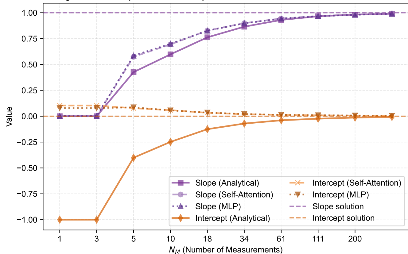
Convergence of Slope and Intercept vs Number of Measurements for 2 Qubits
