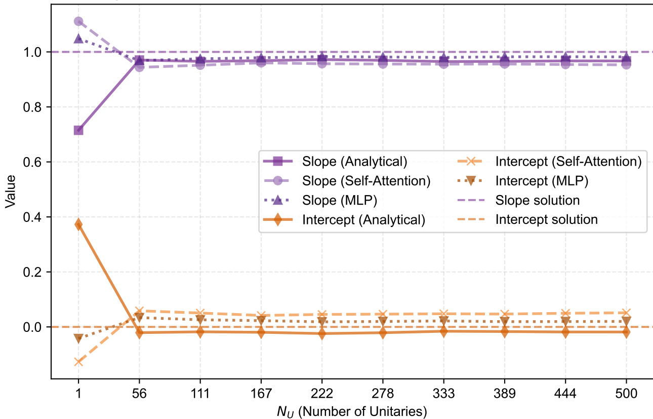
Convergence of Slope and Intercept vs Number of Unitaries for 4 Qubits
