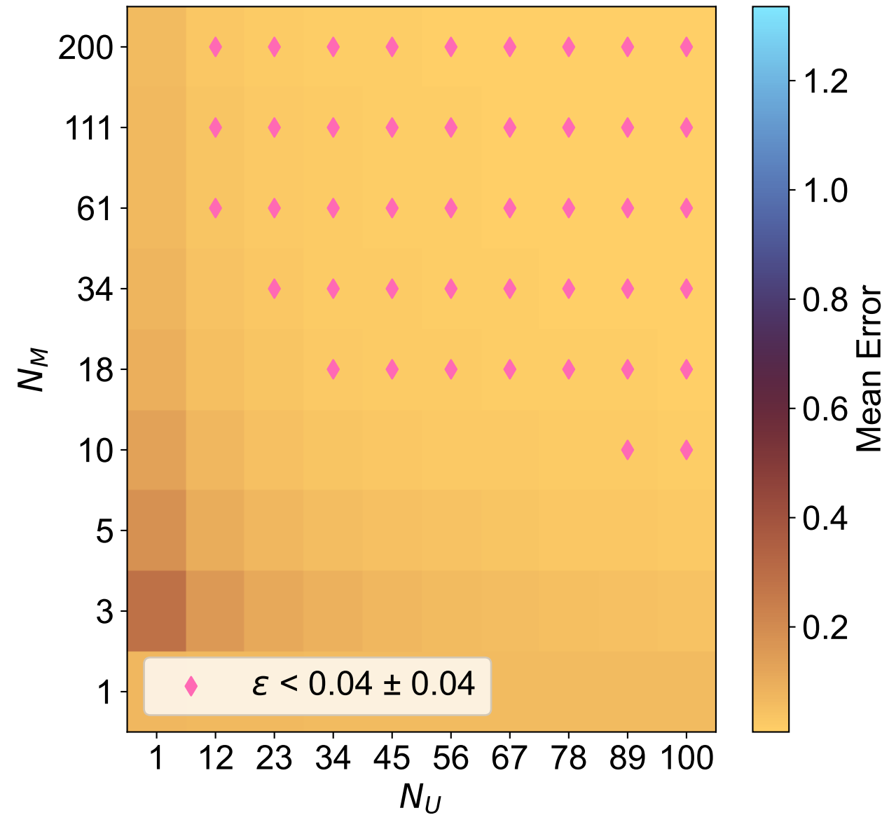
Attention Mean Error Surface
