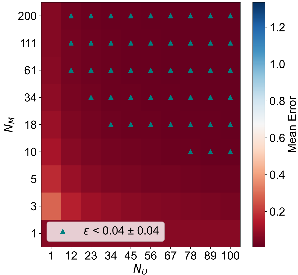
MLP Mean Error Surface
