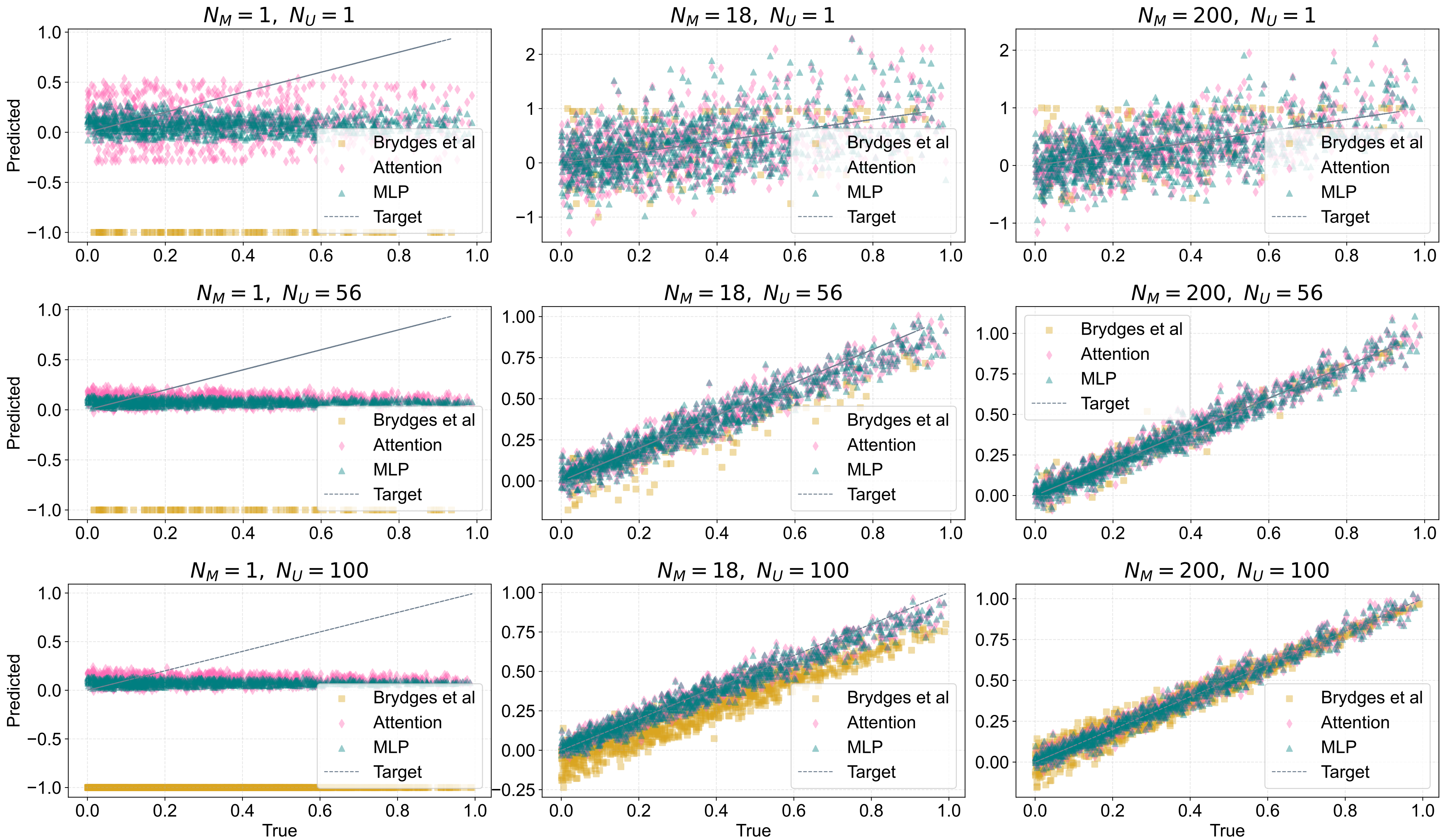
2 Qubits: True vs Predicted Results
