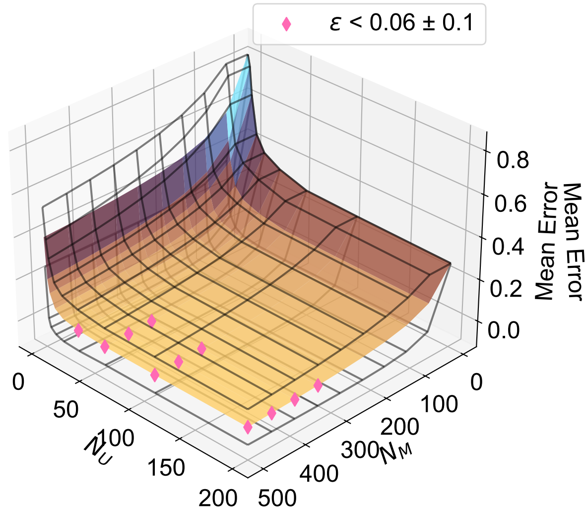
Attention Mean Error Surface
