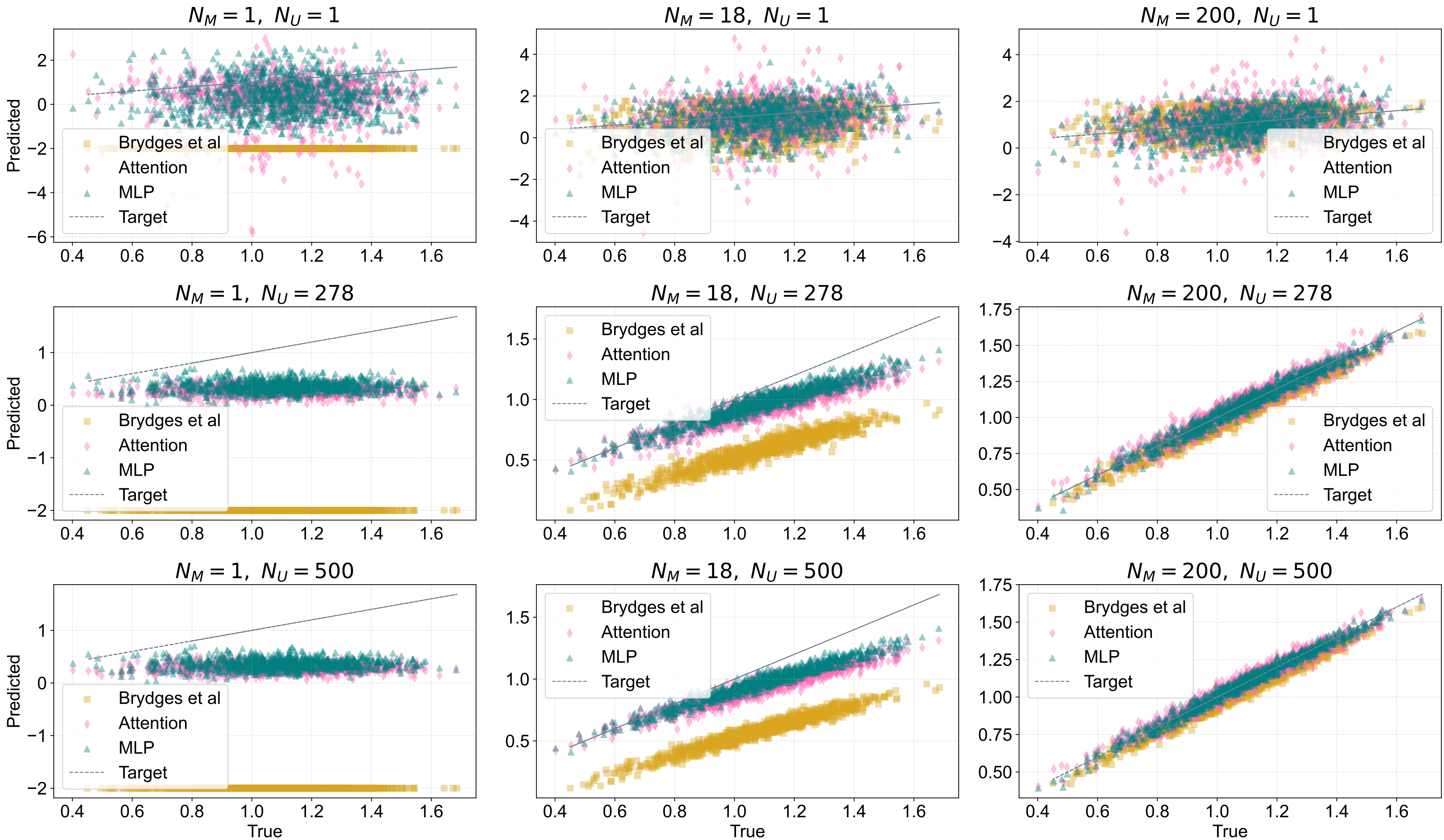
4 Qubits: True vs Predicted Results
