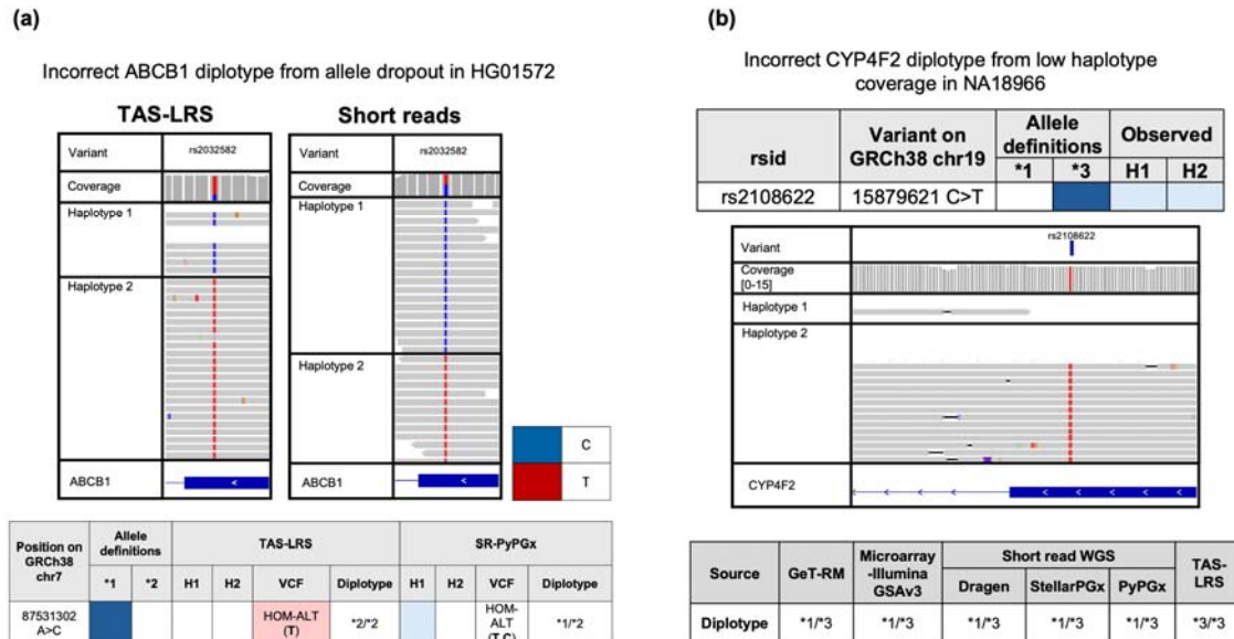
Figure 4 | Examples of discordant calls caused by allele imbalance. (a) Discordant ABCB1 diplotype call in HG01572. rs2032582 was incorrectly called as homozygous alternate (TT) in long-read data, while short-read data supported a heterozygous genotype (TC). The C allele is present in the long reads, but its coverage is too low to meet the variant calling threshold. (b) Discordant CYP4F2 call in sample NA18966. TAS-LRS wrongly called the rs2108622 as homozygous alternate, whereas other platforms including GeT-RM, microarray (GSAv3), and short-read pipelines showed the diplotype as *1/*3. IGV plots show insufficient coverage of haplotype 1 for this specific sample.
