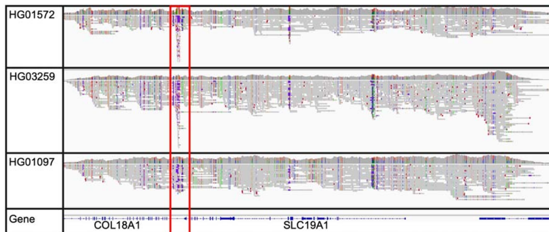
Supplementary Figure 4 | Low-complexity region near SLC19A1 . IGV genome browser plot showing read alignments for three samples (HG01572, HG03259, HG01097) from the 3-plex run “1000ng_cell_lines_5”, highlighting a low-complexity within COL18A1 , located adjacent to SLC19A1 (red box). The gene tracks at the bottom depict the genomic location of COL18A1 (alpha chain of type XVIII collagen) and SLC19A1 . The low-complexity region overlaps with the targeted region for adaptive sampling, and reduces the target coverage for SLC19A1 .
