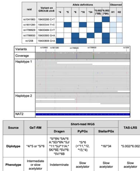
Figure 3 | Examples of improved pharmacogene calls enabled by enhanced phasing, novel allele detection, and expanded haplotype coverage. (a) Phasing and haplotype resolution for NAT2 in NA19174. (b) Improved phasing and detection of a novel allele in CYP2B6 for NA19226. TAS-LRS resolved a partial call (*6/*18 + rs36056539) as the correct genotype.
