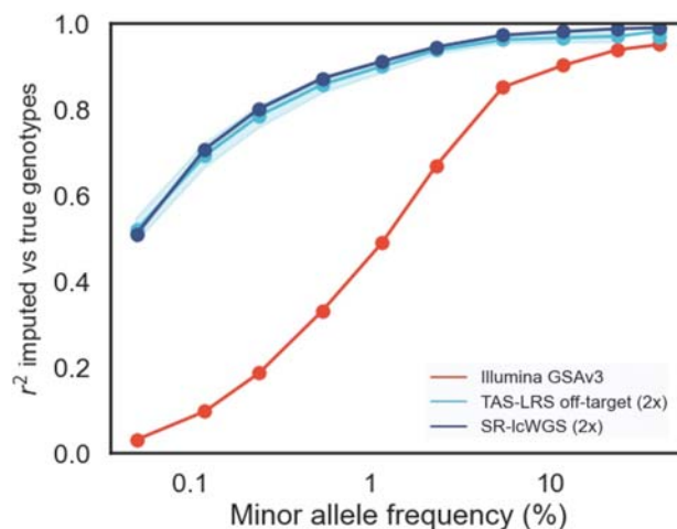
Figure 5 | Genome-wide imputation accuracy across technologies. Imputation was performed using GLIMPSE2 (for TAS-LRS and short-read WGS) and Minimac4 (for microarray data), with the 1KGP reference panel which excludes the test samples (HG002 and HG005 from GIAB). Line plots show imputation accuracy ( R^2 ) across allele frequency bins. Rare variants are defined as those with minor allele frequency <1\% . Shaded areas indicate 95% confidence intervals across replicates.
