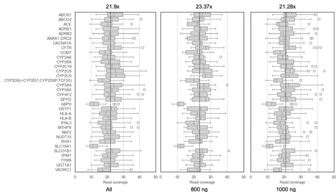
Supplementary Figure 3 | Distribution of read depth in target pharmacogenes. Boxplots representing the distribution of sequencing read depth for 34 pharmacogenes (PGx) targeted in the panel, using a 3-plex adaptive sampling. The dashed vertical line indicates the mean read depth across all genes (21.9x). Most genes demonstrate consistent coverage, while G6PD and SLC19A1 show notably lower coverage across samples. Outliers are depicted as individual points.
