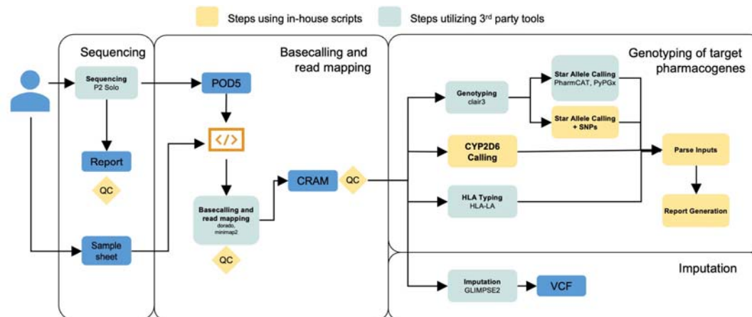
Supplementary Figure 11 | Bioinformatic workflow for pharmacogenomic annotation and genome-wide imputation. Schematic overview of the bioinformatic pipeline, illustrating the steps involved in processing sequencing data for pharmacogenomic analysis. The workflow encompasses sequencing on the ONT P2 Solo platform, basecalling, read mapping, genotyping of target pharmacogenes (including CYP2D6 and HLA typing), and genome-wide imputation using GLIMPSE2. In-house scripts are indicated by orange boxes, while steps utilizing third-party tools are shown in blue. Key file formats - POD5 (raw signal), CRAM (aligned reads), VCF (variant calls) - and quality control (QC) steps are highlighted.
