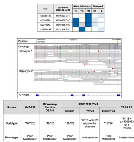
Figure 3 | Examples of improved pharmacogene calls enabled by enhanced phasing, novel allele detection, and expanded haplotype coverage. (a) Phasing and haplotype resolution for NAT2 in NA19174. (b) Improved phasing and detection of a novel allele in CYP2B6 for NA19226. TAS-LRS resolved a partial call (*6/*18 + rs36056539) as the correct genotype.
