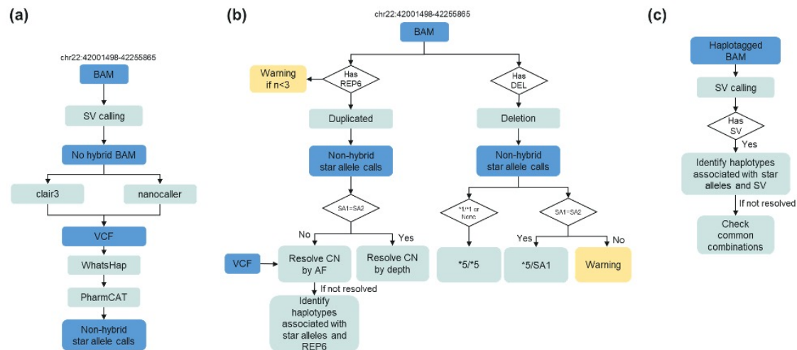
Supplementary Figure 12 | Novel CYP2D6 caller workflow. (a) Schematic outlining the initial variant calling process for CYP2D6 , where non-hybrid reads are used as input for Clair3 and NanoCaller, followed by phasing with WhatsHap and diplotype calling with PharmCAT. (b) Heuristic approach for detecting duplications and deletions in CYP2D6 , including copy number refinement and resolution of complex allele combinations. (c) Heuristic for resolving tandem hybrids, involving structural variant (SV) calling and haplotype association to determine hybrid allele composition.
