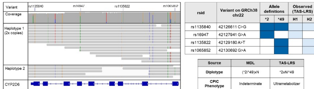
Supplementary Figure 7 | Example of improved CYP2D6 diplotype call leading to refined phenotype classification. IGV genome browser view and variant table for CYP2D6 in sample TTSH_3, showing an example where TAS-LRS resolved a previously unphased copy number change identified by microarrays. This allowed for unambiguous diplotype assignment and a change from 'Indeterminate' to 'Ultrarapid metabolizer' phenotype.
