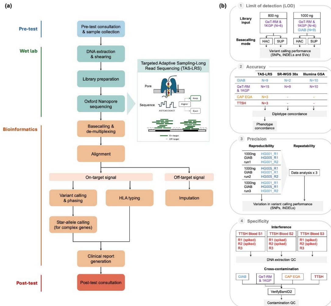
Figure 1 | Overview of the TAS-LRS clinical workflow and validation framework. (a) Schematic of the end-to-end pharmacogenomics testing workflow based on Targeted Adaptive Sampling-Long Read Sequencing (TAS-LRS), comprising four main phases: optional pre-test consultation and sample collection; wet lab processing (DNA extraction, shearing, and Oxford Nanopore sequencing); bioinformatics analysis (including alignment, variant and star-allele calling, HLA typing, and genome-wide imputation); and post-test clinical consultation. Adaptive sampling enriches for 35 target pharmacogenes, including all PharmGKB Very Important Pharmacogenes (VIPs) and HLA-A, while generating low-depth off-target data for broader genome-wide applications. Blue, green, orange, and red indicate distinct workflow stages. (b) Validation framework for the TAS-LRS workflow, consisting of four core studies: (1) Limit of Detection (LOD), evaluating variant calling performance (SNVs, indels, and SVs) across different DNA input amounts (800 ng vs 1000 ng) and basecalling models (High-accuracy (HAC) vs Super-accuracy (SUP)); (2) Accuracy, assessed by
