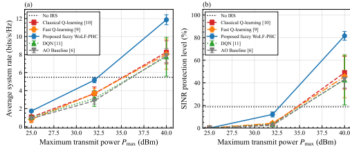
Fig. 2. (a) System rate and (b) SINR protection vs. maximum transmit power P_{\max} ; WoLF-PHC scales most effectively with power.
