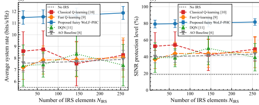
Fig. 3. (a) System rate and (b) SINR protection vs. IRS array size N_{\text{IRS}} ; gains grow but saturate near N_{\text{IRS}} = 256 .
