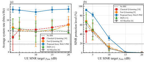
Fig. 4. (a) System rate and (b) SINR protection vs. UE SINR target \gamma_{\min} ; WoLF-PHC degrades most gracefully.
