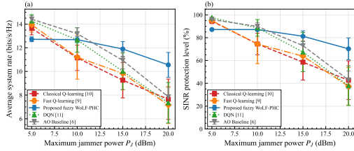
Fig. 5. (a) System rate and (b) SINR protection vs. maximum jammer power P_J ; a regime transition occurs near 10–15 dBm.
