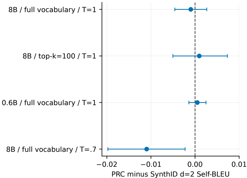
A Paired Self-BLEU difference Negative favors PRC
