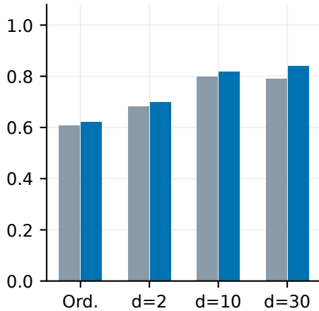
Maximum token probability
