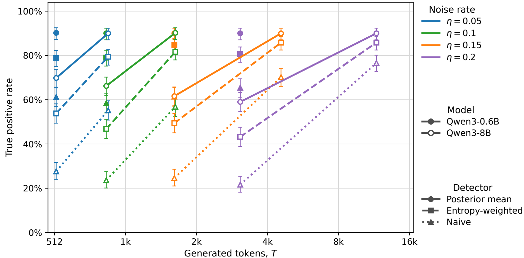
Detection power (Online PRC)
