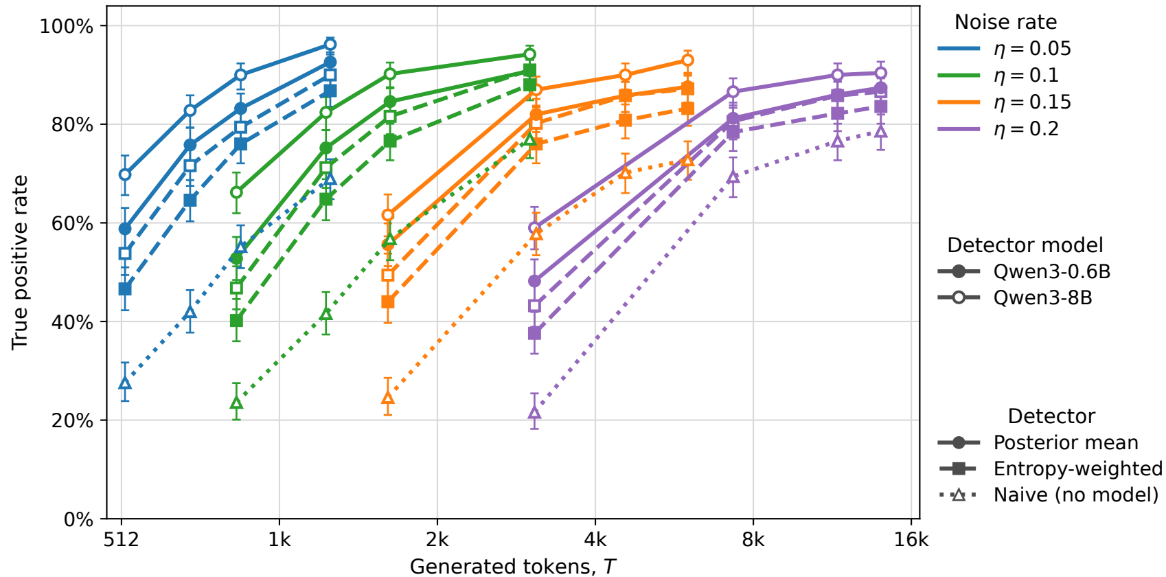
Same-model vs. cross-model watermark detection
