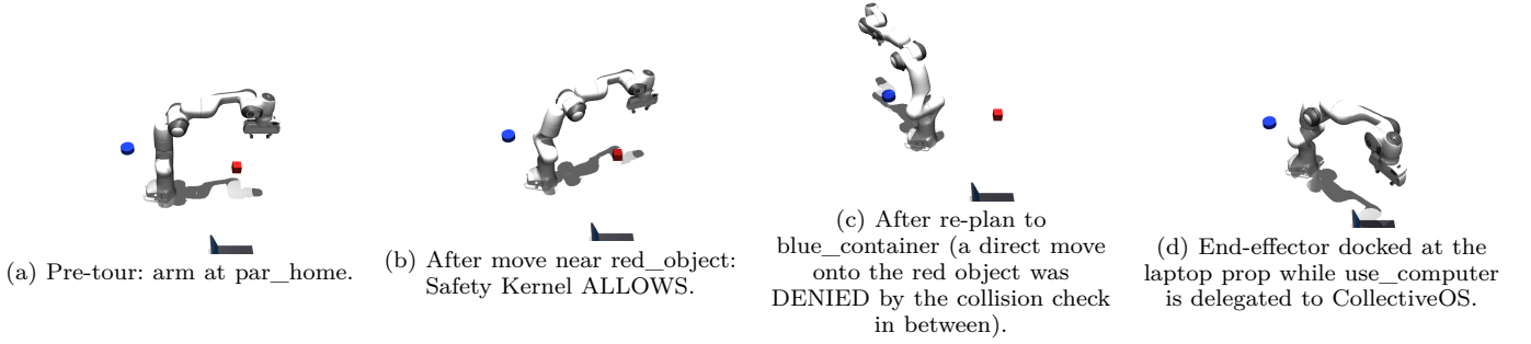
Fig. 2. Four moments from a single real end-to-end run of the arena tour example (examples/mujoco_loop.py): a Franka Emika Panda arm in MuJoCo being driven by Pulse’s scripted planner through the Safety Kernel. Panel (c) is the clearest visual evidence of the governance behavior the paper describes: between (b) and (c) a proposed move straight onto red_object was denied by the Safety Kernel’s collision-margin check, so no arm motion occurred for that step; the planner re-planned to the blue container next. Panel (d) shows the begin_computer_use hook docking the arm at the laptop prop for the duration of the delegation to CollectiveOS, making the hand-off a visible physical gesture rather than an invisible RPC. Frames rendered via mujoco.Renderer inside the bridge process; the exact camera is MuJoCo’s default free camera, with no post-processing.
