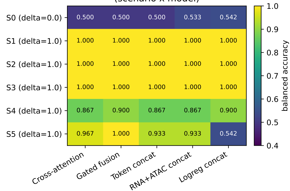
Planted benchmark: balanced accuracy (scenario x model)
