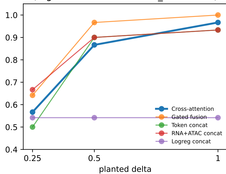
S5: balanced accuracy vs delta (regime at delta=1.0: MLP_FAVOURED)
