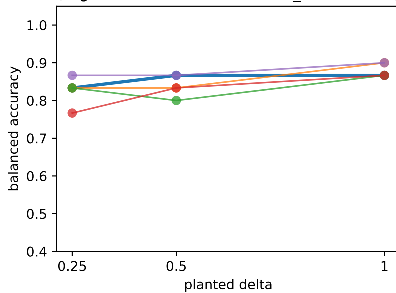
S4: balanced accuracy vs delta (regime at delta=1.0: LINEAR_SUFFICIENT)
