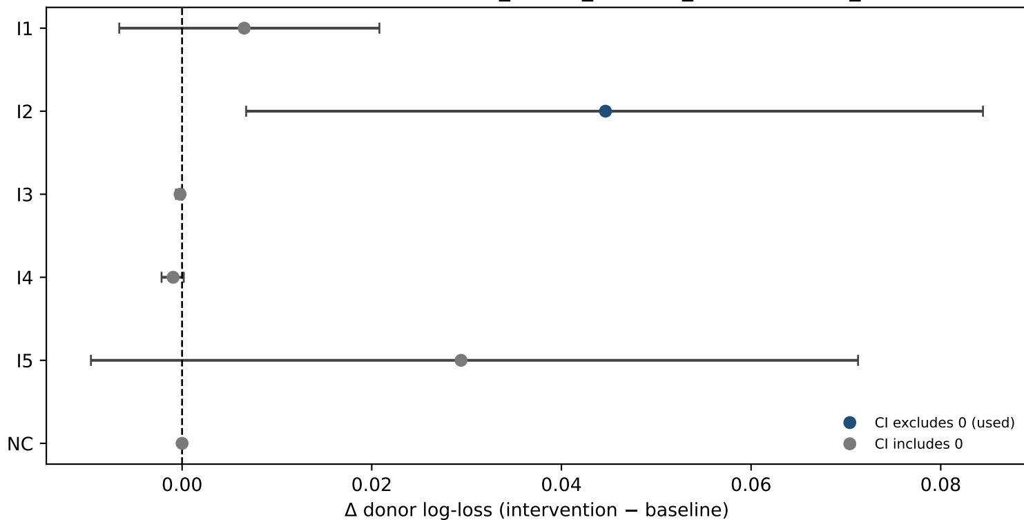
Faithfulness interventions on R3_ca (CA_PAIRING_UNUSED, ATAC_USED)
