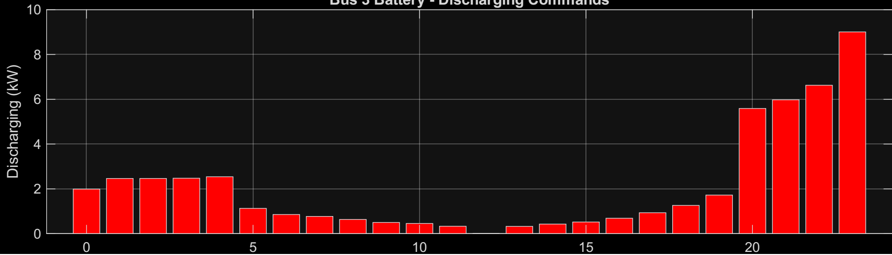
Bus 3 Battery - Discharging Commands
