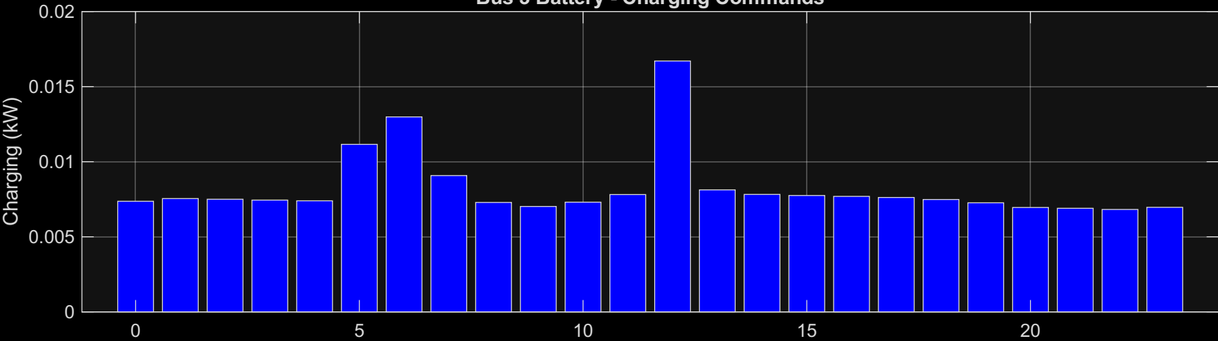
Bus 3 Battery - Charging Commands
