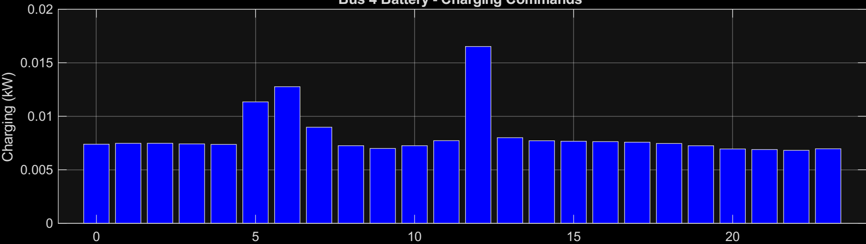
Bus 4 Battery - Charging Commands
