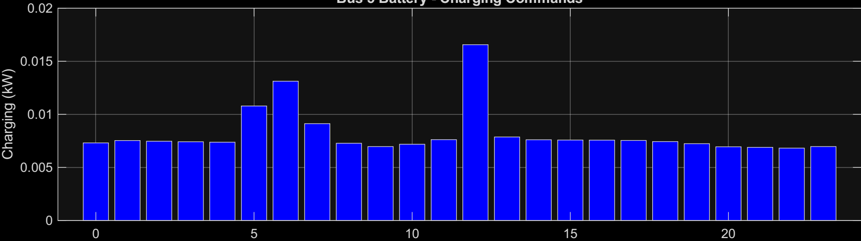
Bus 5 Battery - Charging Commands
