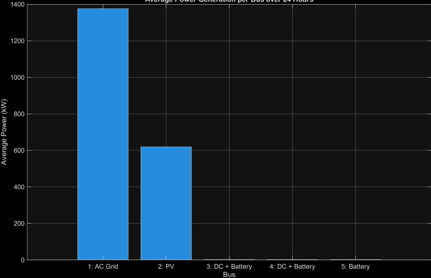
Average Power Generation per Bus over 24 Hours
