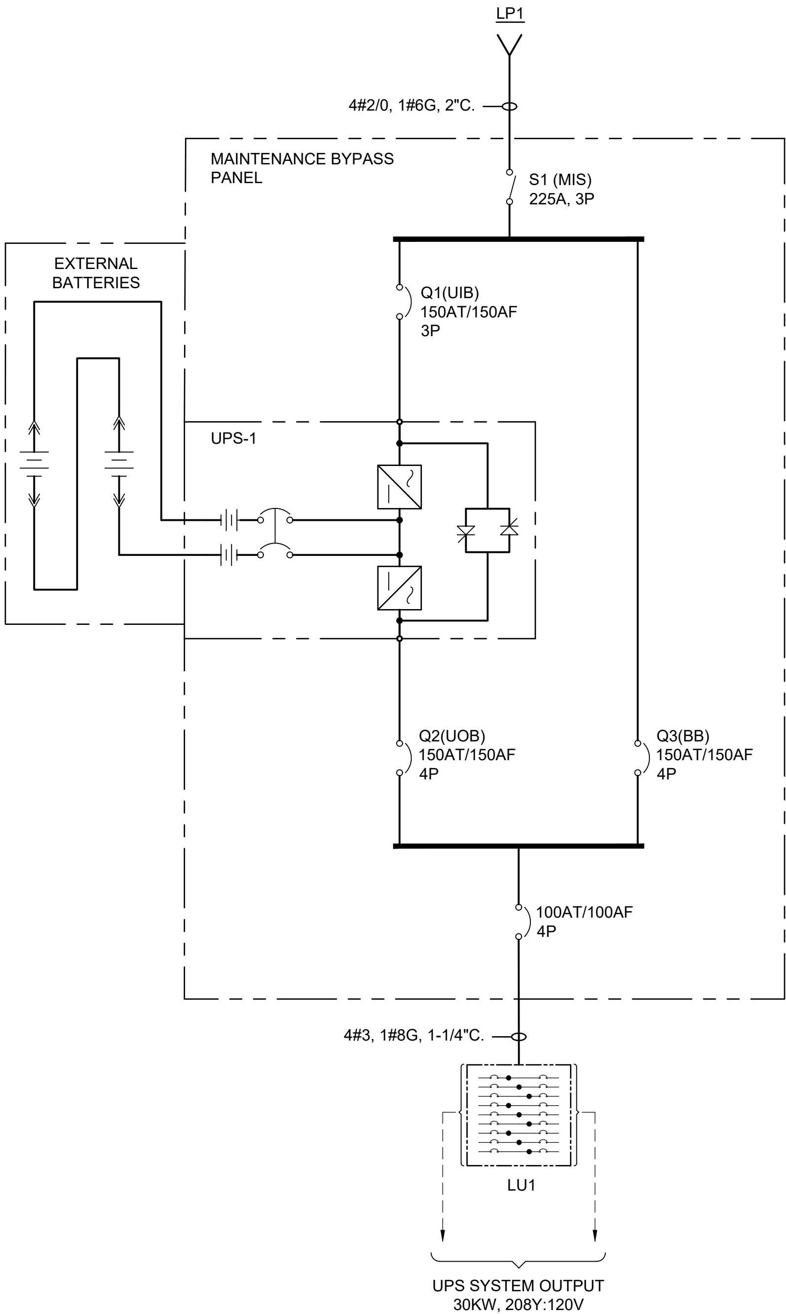
UNINTERRUPTIBLE POWER SUPPLY UPS-1 ONE-LINE DIAGRAM NTS
