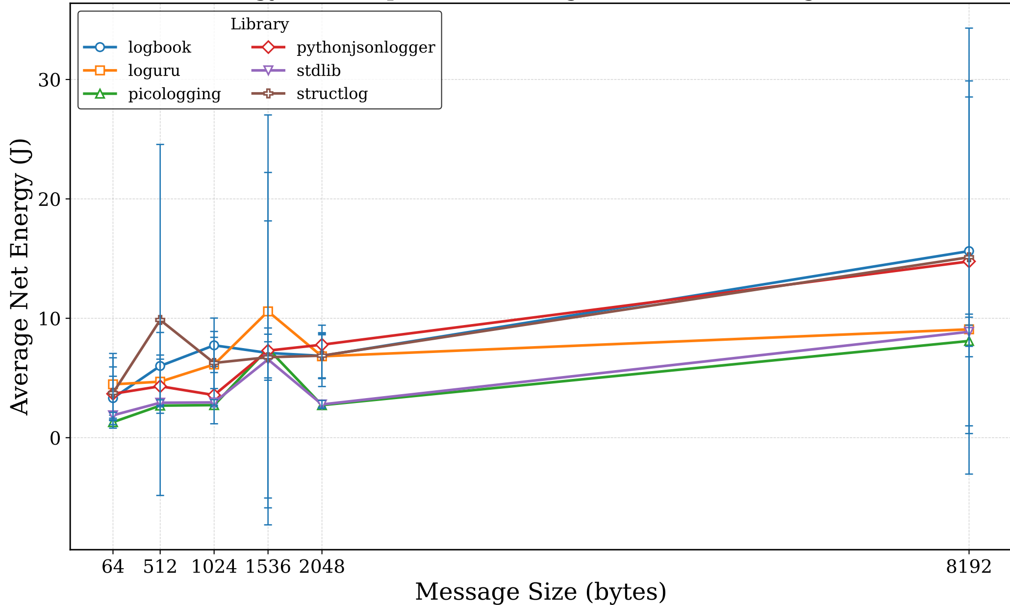
Energy Consumption vs Message Size (Rate = 1 logs/sec)
