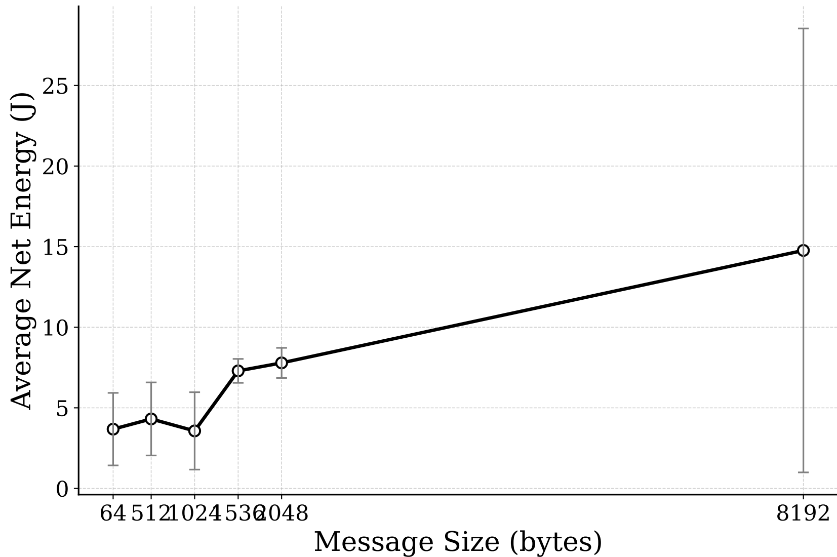
pythonjsonlogger (Rate = 1 logs/sec)
