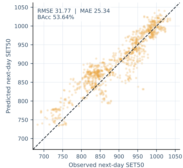
LSTM-CNN-Attention
