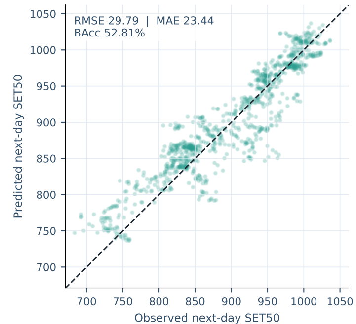
LSTM-CNN
