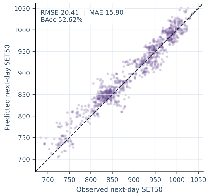
LSTM-Attention
