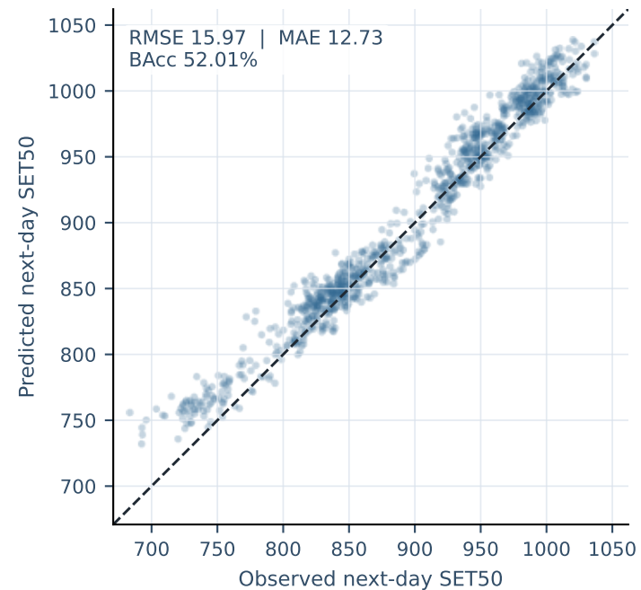
LSTM
