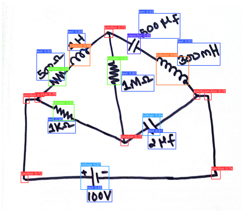
Figure 6-12 Retrained YOLOv7 Result (i)
