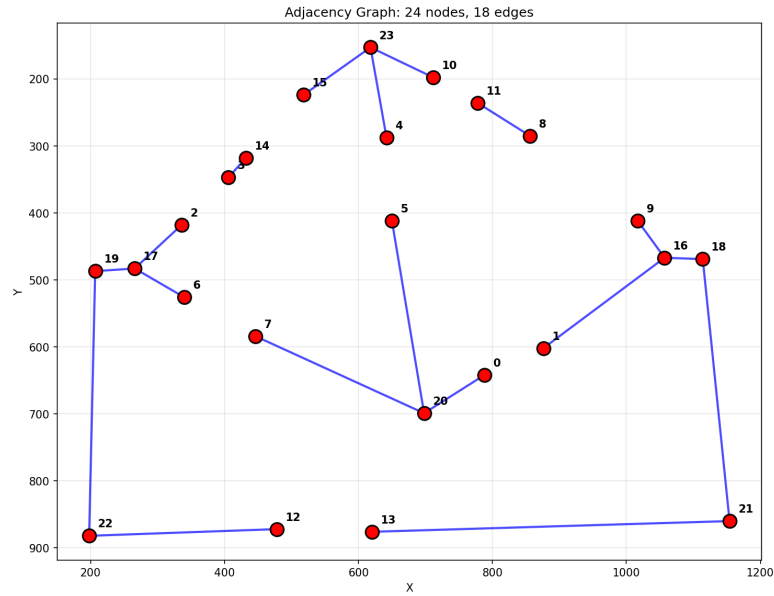
Figure 6-24 Adjacency graph constructed using Multi-Head BFS algorithm
