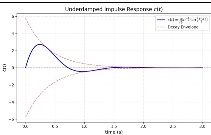
Fig. 1.2.6.1. c(t) vs time
