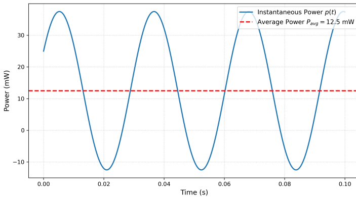
Fig. 1.2.11.1. Power vs time
