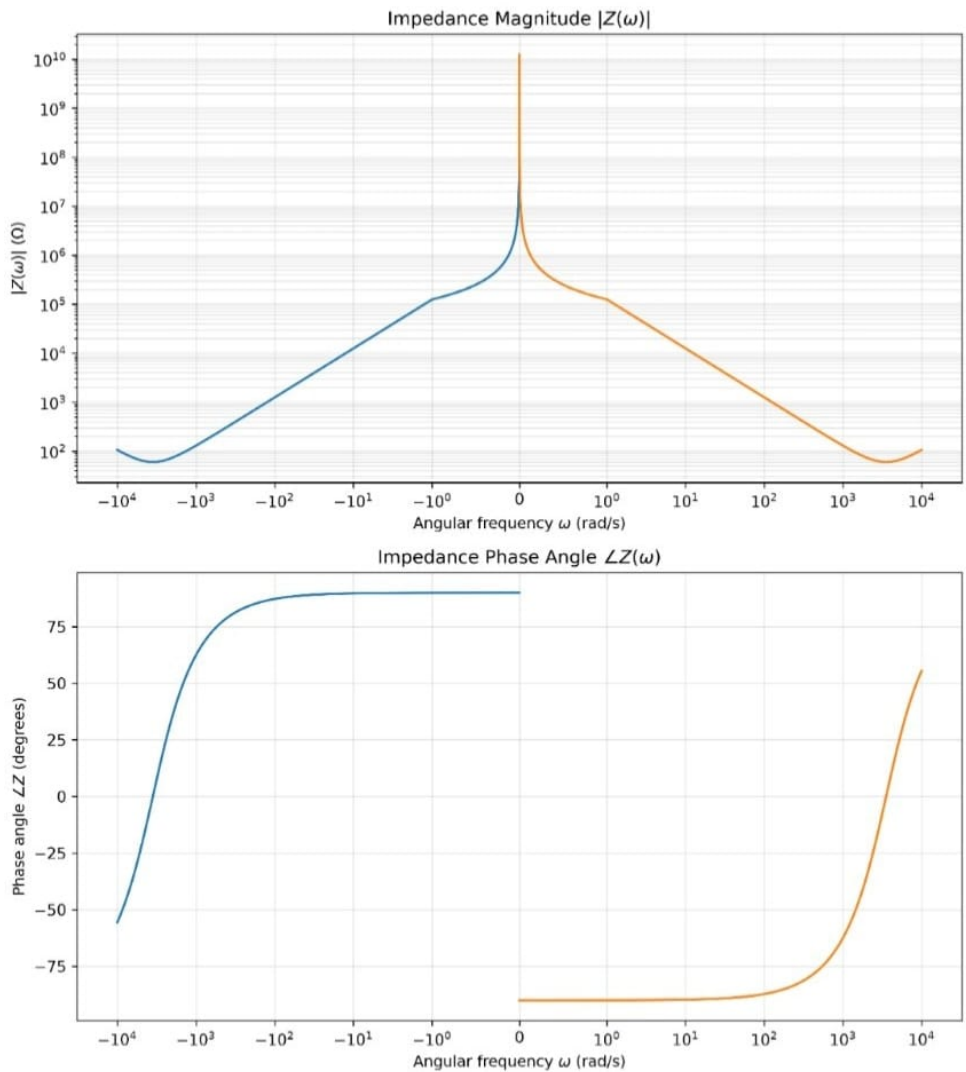
Fig. 1.2.21.1. Impedence mag vs angular frequency, Impedence phase angle vs angular frequency
