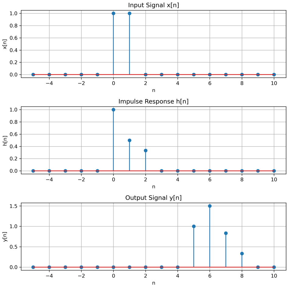
Fig. 1.0.17.1. x[n], h[n], y[n] vs n
