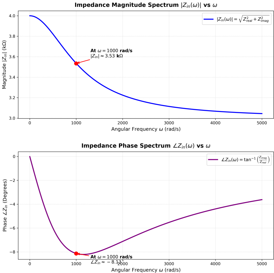
Fig. 1.0.14.1. Impedance Magnitude VS Omega; Phase VS Omega
