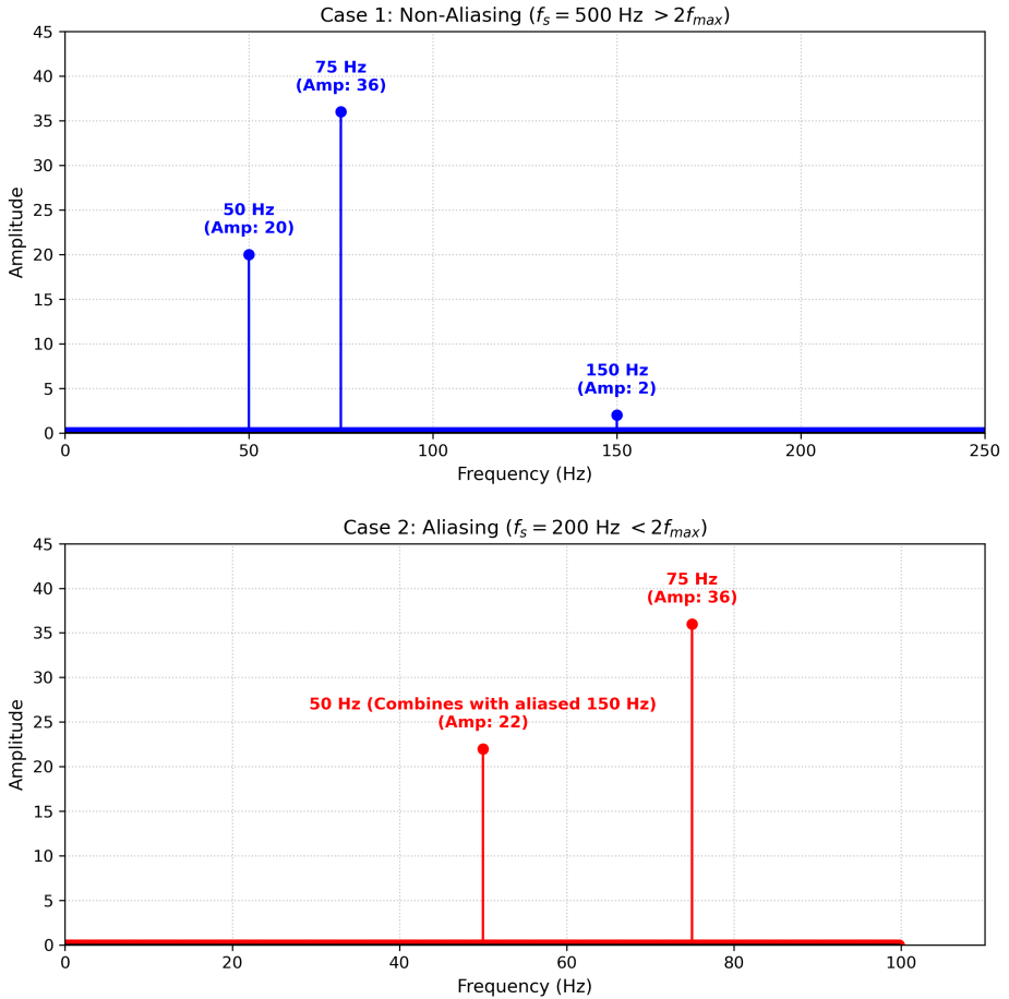
Fig. 1.0.10.1. Aliasing and Non-Aliasing
