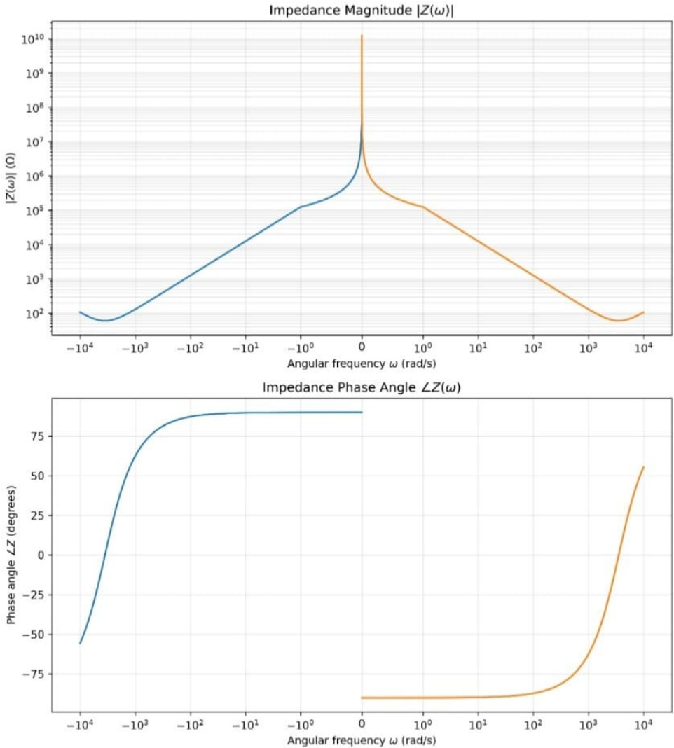
Fig. 1.0.21.1. Impedance mag vs angular frequency, Impedance phase angle vs angular frequency
